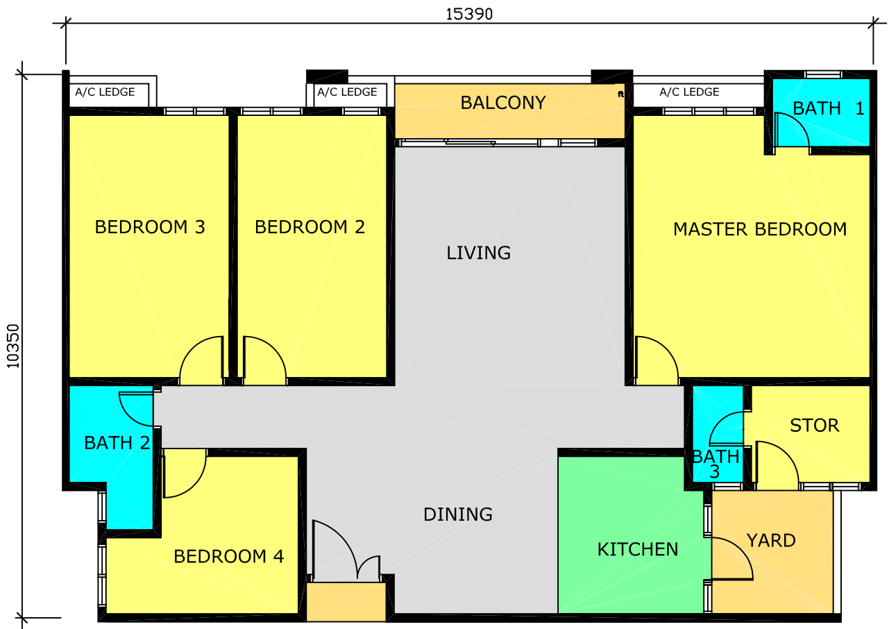
TYPE D ( 1,589 sqft. )
